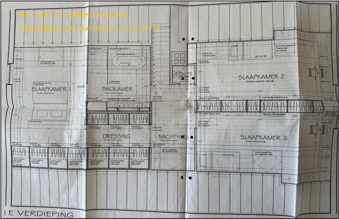
Legende van plan 1.2: Plan V1
